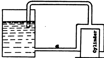
FIG. 41.—Thermo-Syphon System.
